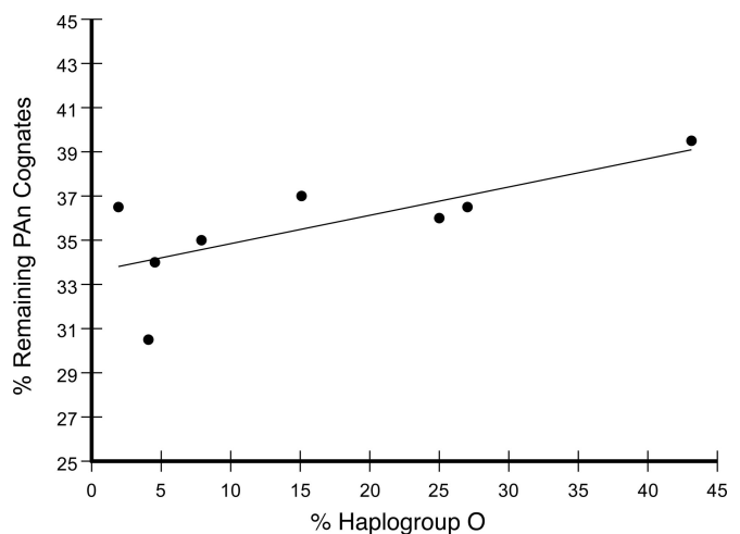
Fig. 3. Scatterplot of the percentage of PAN cognates versus the percentage of Austronesian Y chromosomes (haplogroup O) found at each location.
